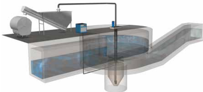
Illustration Noggerath® Rundsandfang Vortex GCC-V
