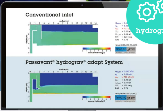
Virtual Capacity Simulation STP
